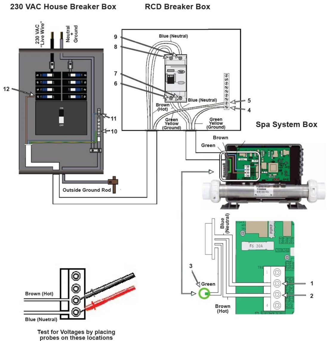
Figure 4. Wiring Schematic for 50 Hz Systems
